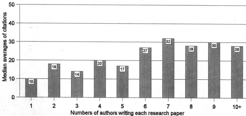
FIGURE 2 Median averages of citations received, organized by the number of researchers authoring each paper.
