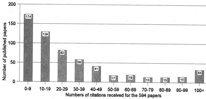
FIGURE 1 Frequency distributions of citations for animal-based research studies published by HSC-affiliated authors between 1990 and 1995.
